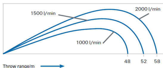
Throw Range at 8 bar
