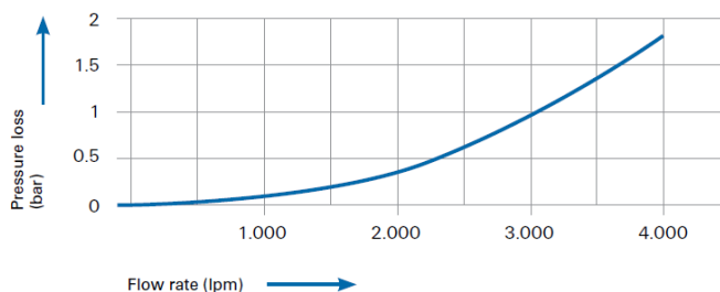
Pressure vs. Throw Range - TWISTER P/O
